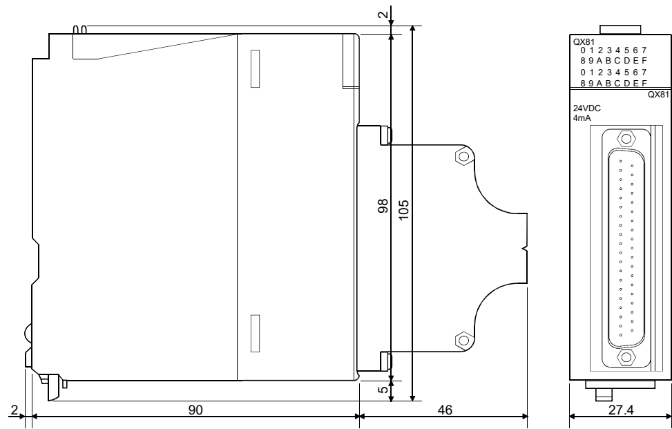
(4) 37-pin D-sub connector type 32-point I/O module
