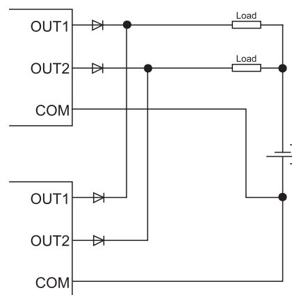
Source type
