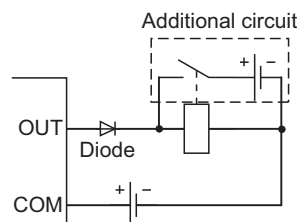
Source type
