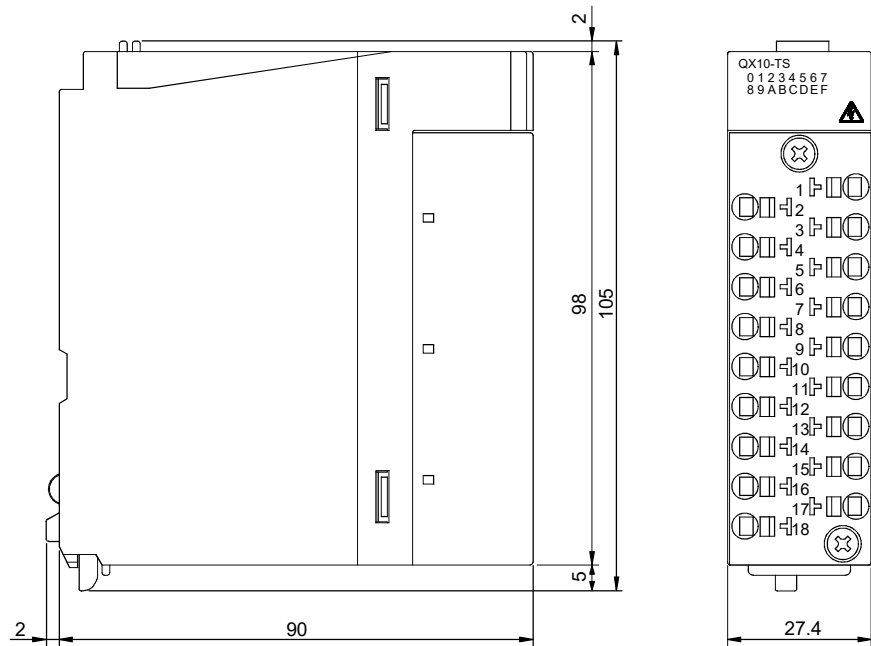
(2) Spring clamp terminal block type
