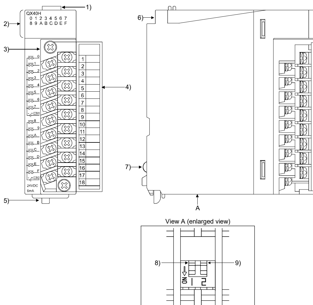
18-point screw terminal block type (high-speed input module)
