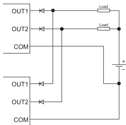
Sink type
