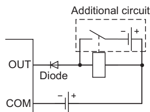
Sink type
