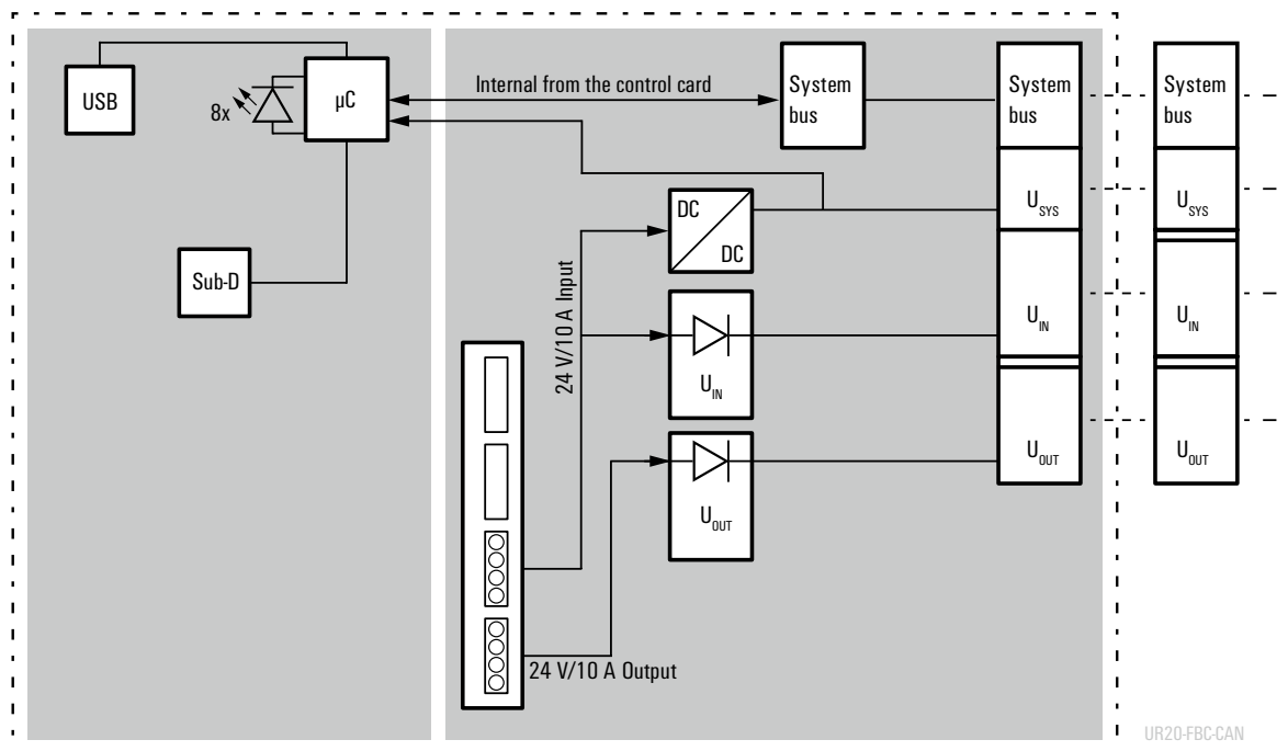
电路框图：UR20-FBC-CAN
